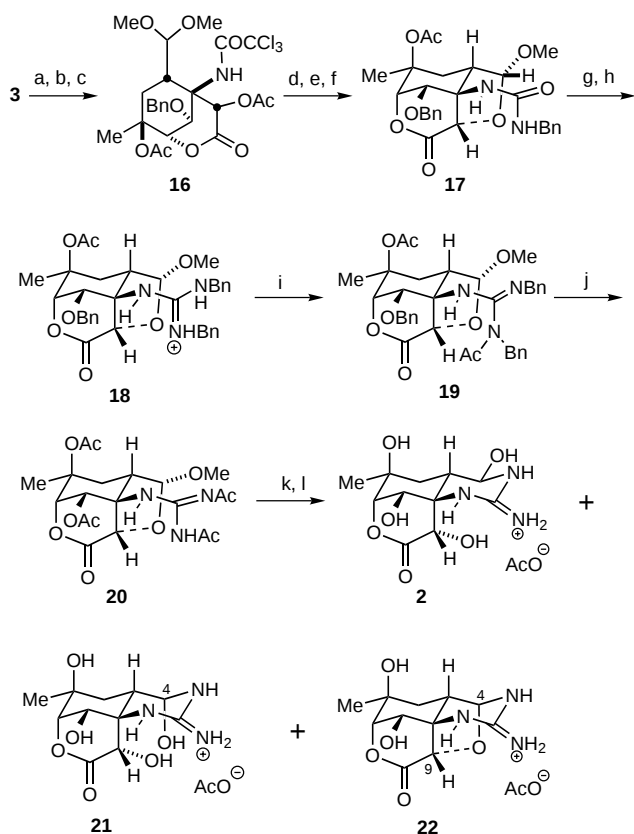
Scheme 3. Synthesis of 5,11-dideoxytetrodotoxin (2). a) \text{H}_5\text{IO}_6 , \text{AcOEt} , rt, 24 h; b) CSA, \text{CH}(\text{OMe})_3 , MeOH, rt, 10 h; c) \text{Ac}_2\text{O} , pyridine, DMAP, rt, 24 h, 78 % over three steps; d) \text{BnNH}_2 , \text{Na}_2\text{CO}_3 , DMF, 140^\circ\text{C} , 15 min; e) KCN, EtOH, rt, 1 h; f) CSA, acetone, rt, 2 h, 70 % over three steps; g) \text{Ph}_3\text{P} , \text{CBr}_4 , \text{Et}_3\text{N} , \text{CH}_2\text{Cl}_2 , rt, 4 h; h) \text{BnNH}_2 \cdot \text{HCl} , pyridine, reflux, 5.5 h; i) \text{Ac}_2\text{O} , pyridine, \text{Et}_3\text{N} , rt, 4.5 h, 85 % over three steps; j) \text{H}_2 (1 atm), \text{Pd}(\text{OH})_2/\text{C} , \text{Ac}_2\text{O} , rt, 14 d, 81 %; k) aq. \text{NH}_3 , MeOH– \text{H}_2\text{O} , rt, 20 h; l) TFA, \text{H}_2\text{O} , rt, 34 h, 81 % over two steps. CSA = 10-camphorsulfonic acid, DMAP = 4-dimethylaminopyridine, TFA = trifluoroacetic acid.
