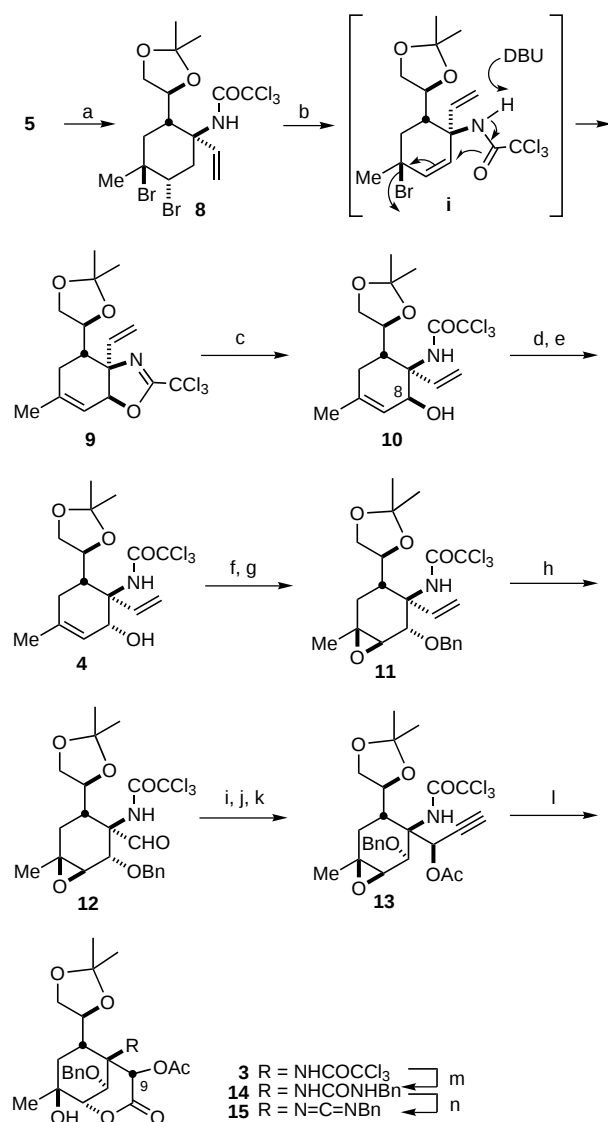
Scheme 2. Synthesis of lactone 15 . a) Pyridinium bromide perbromide, K 2 CO 3 , CH 2 Cl 2 , 10 °C, 3 h, 87%; b) DBU, DMF, rt, 6 h; c) p TsOH, pyridine–H 2 O, 70 °C, 1.5 h, 71 % over two steps; d) PCC, MS 4 Å, CH 2 Cl 2 , rt, 11 h; e) NaBH 4 , CeCl 3 (H 2 O) 7 , EtOH–CH 2 Cl 2 , 0 °C, 2 h, →rt, 30 min, 75 % over two steps; f) MCPBA, CH 2 Cl 2 , rt, 24 h; g) NaH, BnBr, THF–DMF, rt, 22 h, 86 % over two steps; h) O 3 , MeOH, –78 °C, 70 min, Me 2 S, 96 %; i) Me 3 SiC≡CMgBr, THF, rt, 2 h; j) n Bu 4 NF, THF, rt, 2.5 h; k) Ac 2 O, pyridine, rt, 5.5 h, 86 % over three steps; l) RuO 2 (H 2 O) m , NaIO 4 , CCl 4 –CH 3 CN–H 2 O, rt, 4.5 h, 75 %; m) BnNH 2 , Na 2 CO 3 , DMF, 125 °C, 30 min; n) Ph 3 P, CBr 4 , Et 3 N, CH 2 Cl 2 , rt, 7 h, 87 % over two steps. DBU = 1,8-diazabicyclo[5.4.0]undec-7-ene, DMF = dimethylformamide, rt = room temperature, p TsOH = 4-toluenesulfonic acid, PCC = pyridinium chlorochromate, MCPBA = meta -chloroperbenzoic acid.
